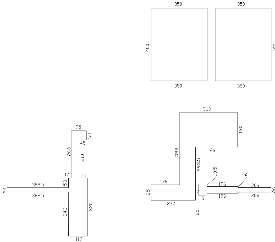
CIRCUIT DIMENSIONS
