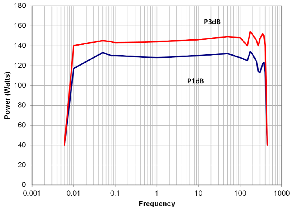
125A400 Typical Power Output
