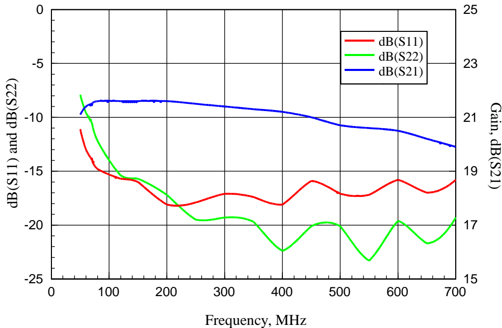
ABL0050-20-2008 Measured Gain and Return Loss vs Frequency
