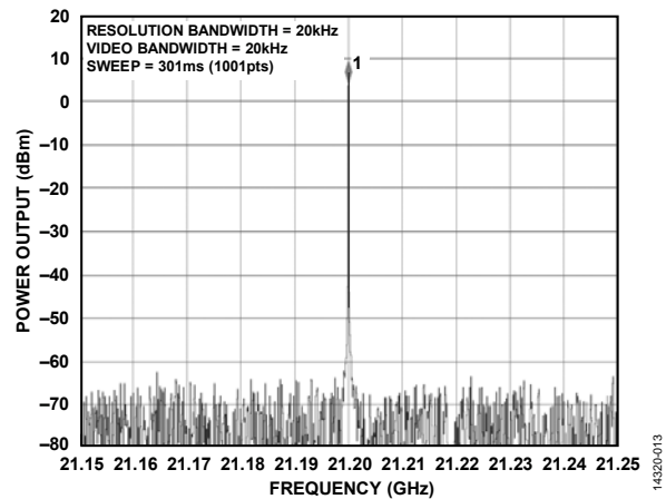
Figure 18. Test Results at 21.2 GHz
