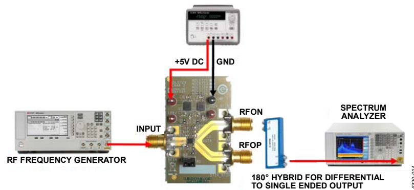
Figure 19. ADL5726-EVALZ Lab Bench Setup
