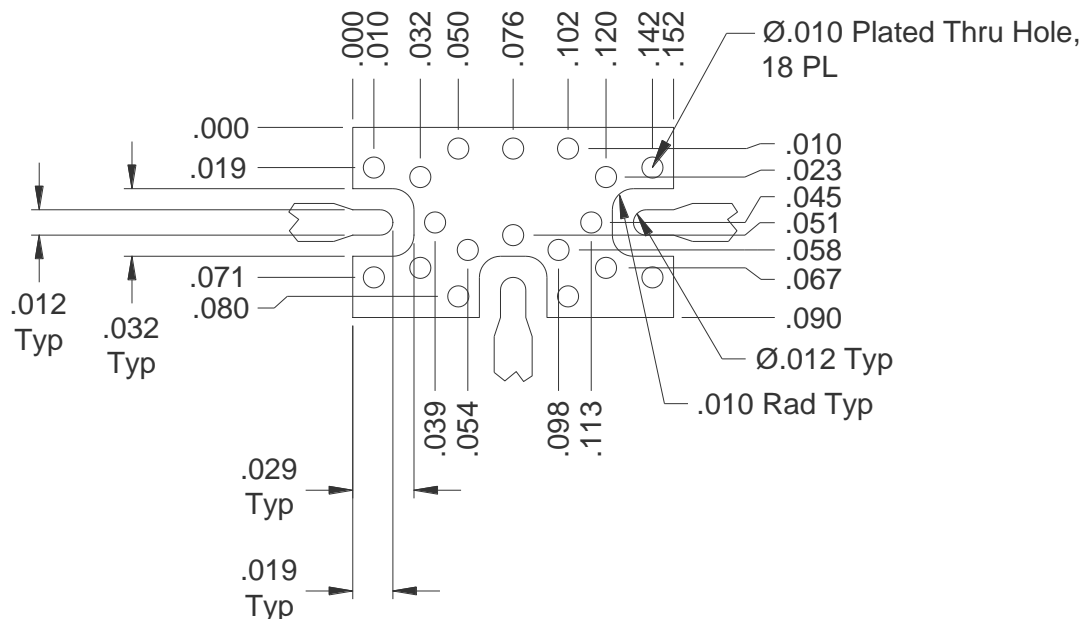
Outline Drawing – SM-2 and SM-1 Packages
