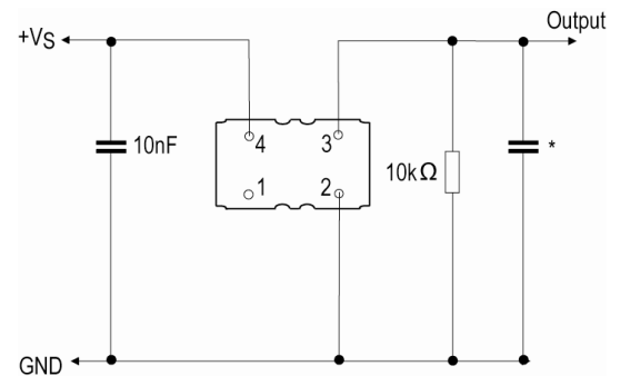
Test Circuit
