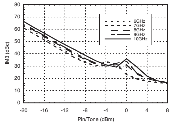
Output IM3, 7V @ 820 mA
