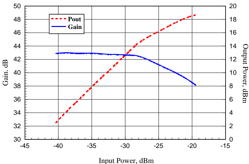
ABL0600-01-4345 Measured Gain and Output Power vs Input Power Test Frequency: 100MHz
