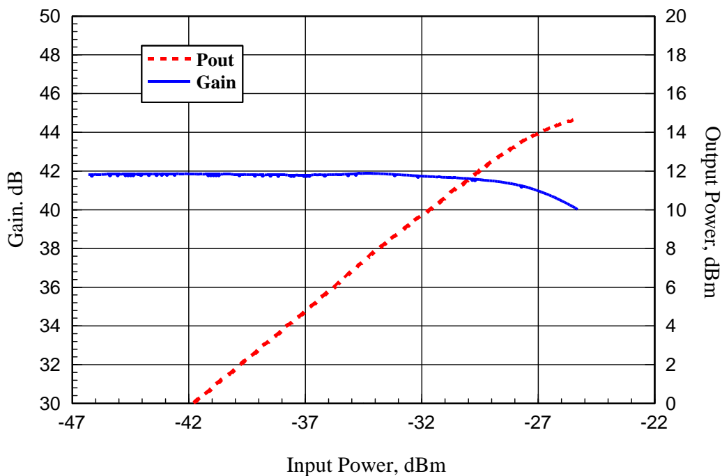
ABL0600-01-4345 Measured Gain and Output Power vs Input Power Test Frequency: 6000MHz
