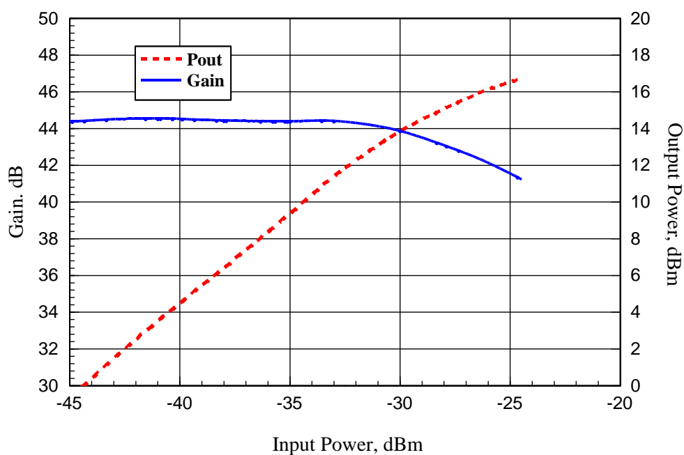
ABL0600-01-4345 Measured Gain and Output Power vs Input Power Test Frequency: 3000MHz
