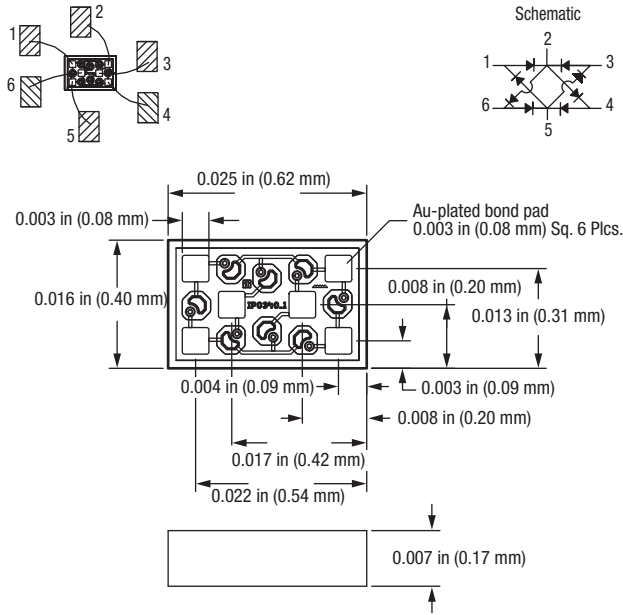
Figure 6. 588-065 Package Dimensions
