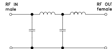
electrical schematic
