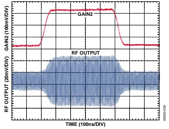
Figure 33. V_{GAIN} Step Response (VGA Mode) over Gain Step, V_{IN} = 100 mV p-p for VGA2
