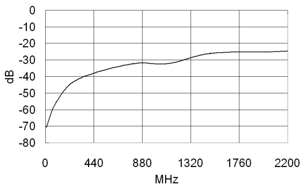
LO-IF Isolation
