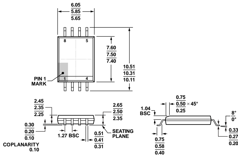
Figure 24. 8-Lead Standard Small Outline Package, with Increased Creepage [SOIC_IC] Wide Body (RI-8-1) Dimensions shown in millimeters
