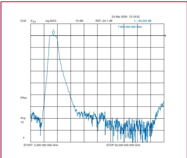
5IB10-7800 Outer Band Rejection
