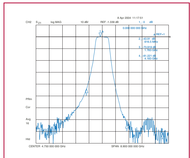
5IB10-4750 Outer Band Rejection
