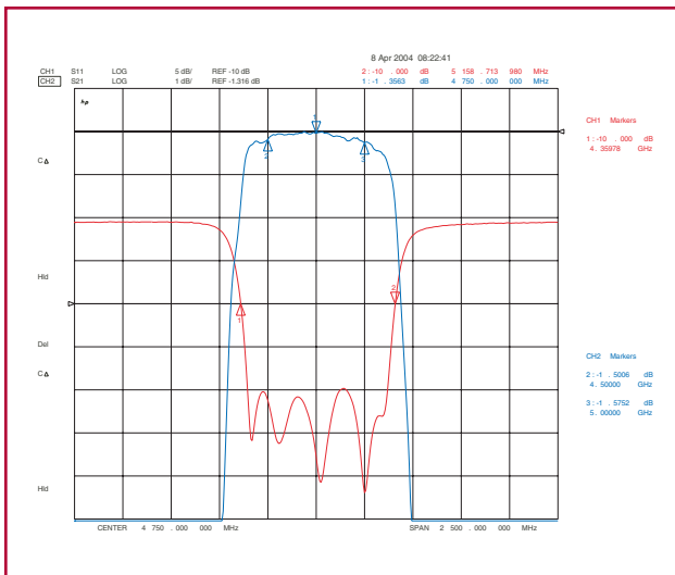
5IB10-4750 Passband
