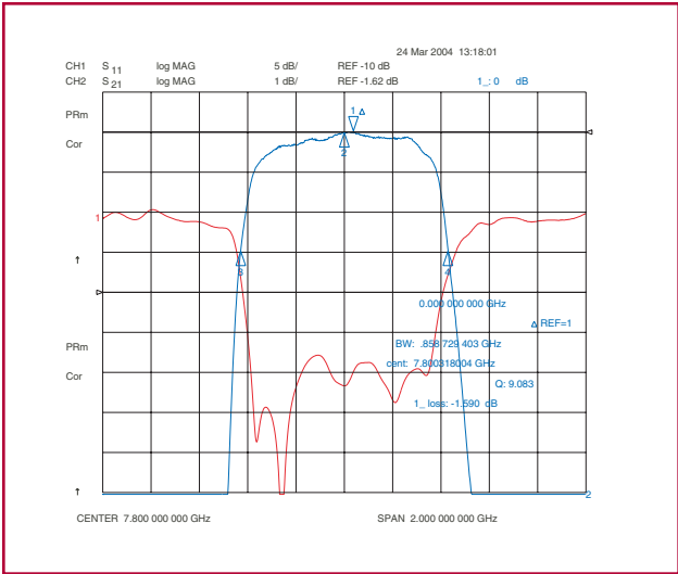
5IB10-7800 Passband
