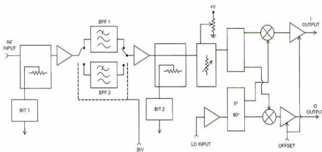
IQ - DETECTOR MODULE BLOCK DIAGRAM
