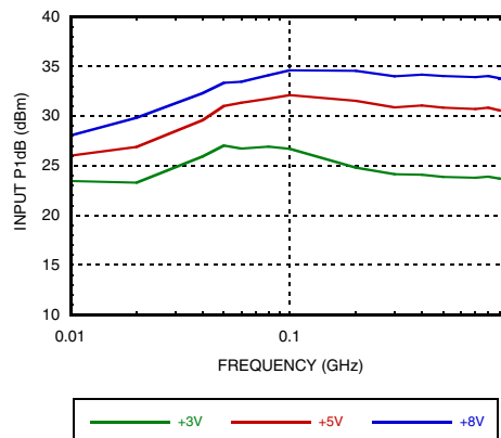
Low Frequency Input P1dB vs. Vctl
