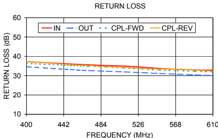
SYBD-26-62HP+ RETURN LOSS
