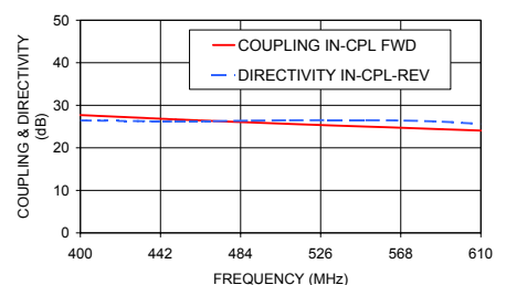
SYBD-26-62HP+ COUPLING & DIRECTIVITY
