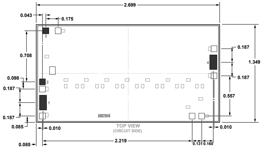
Figure 36. 4-Pad Bare Die [CHIP] (C-4-1) Dimensions shown in millimeters
