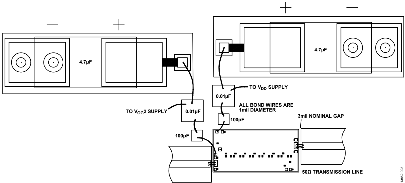
Figure 35. Assembly Diagram
