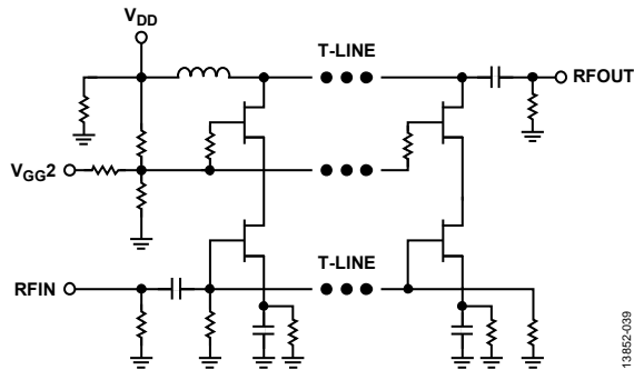
Figure 32. Architecture and Simplified Schematic
