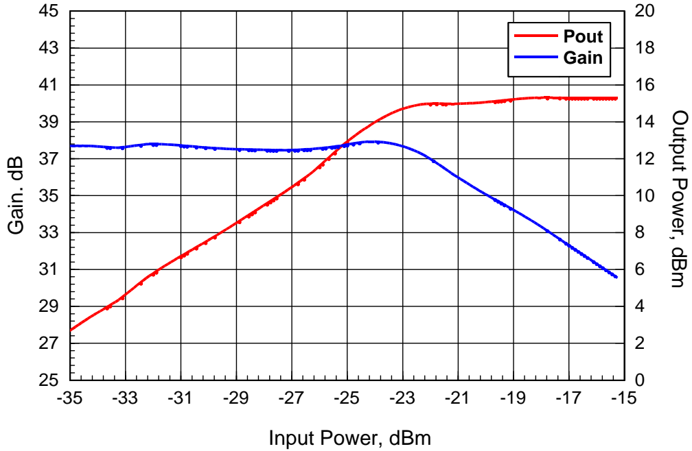
ABL0400-25-3715 Measured Gain and Output Power vs Input Power Test Frequency: 1000MHz
