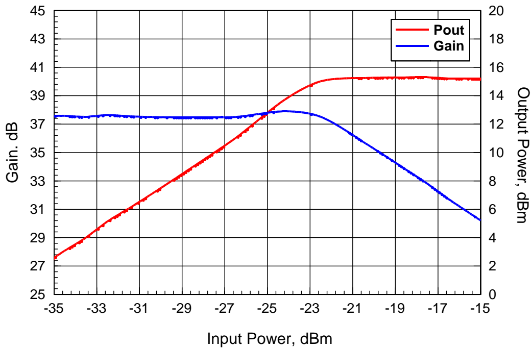
ABL0400-25-3715 Measured Gain and Output Power vs Input Power Test Frequency: 2500MHz
