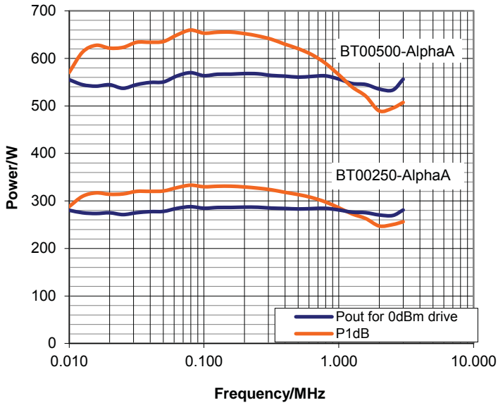
Typical peak output power plots
