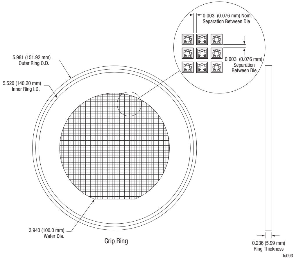
Figure 3. Wafer on Film
