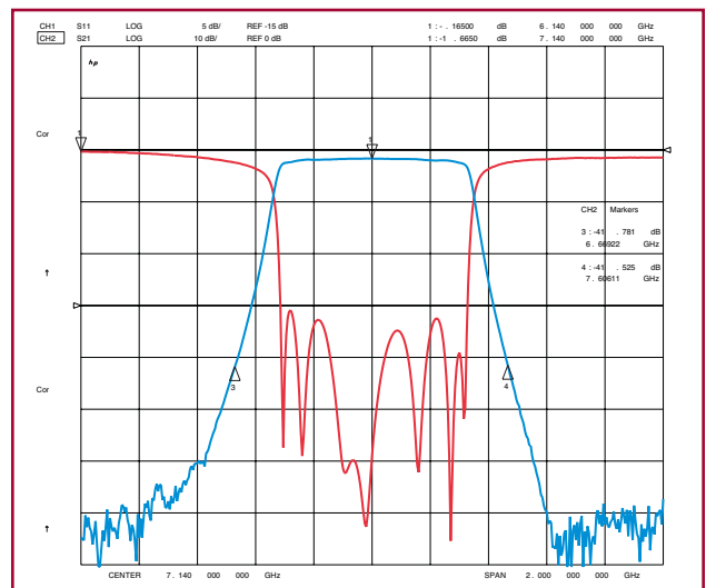
40 dB Rejection Points
