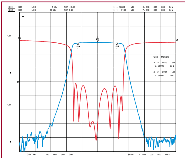
Insertion Loss Characteristics
