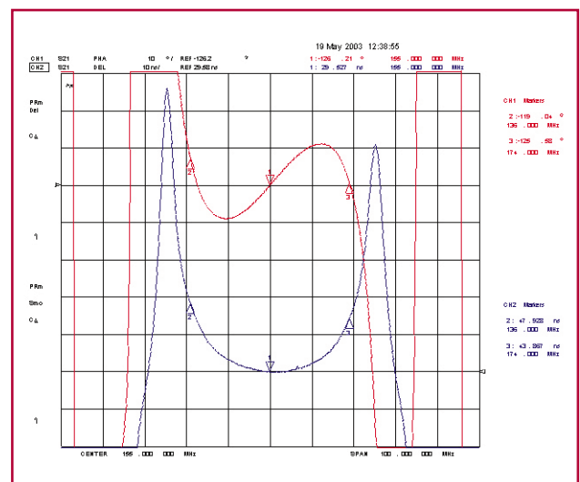
Phase/Group Delay
