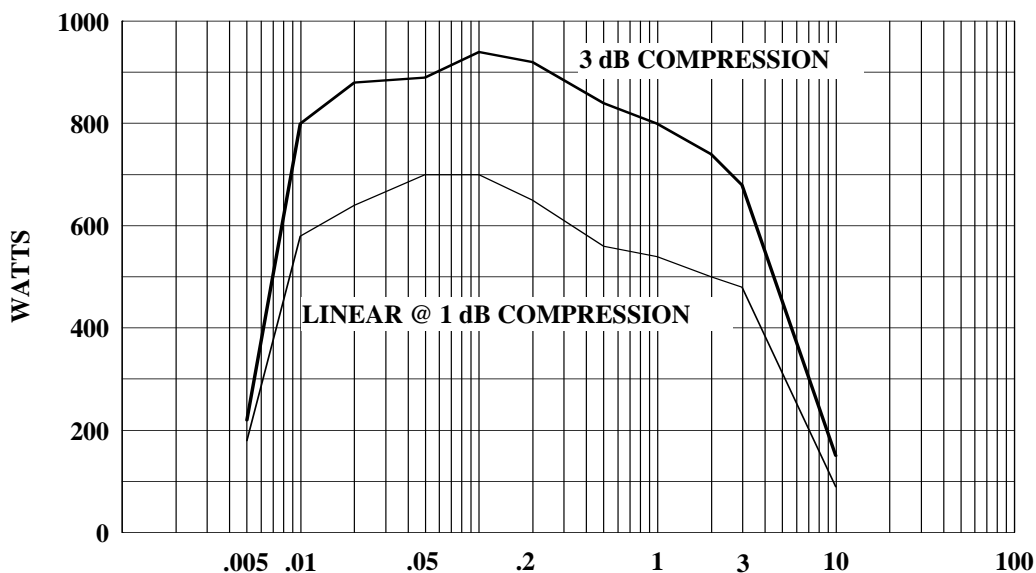
800A3A TYPICAL POWER OUTPUT
