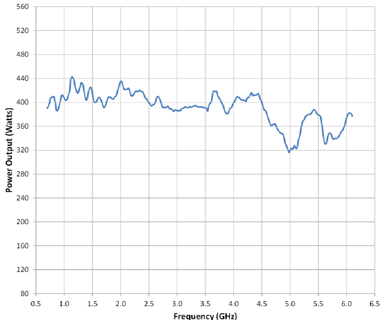
300S1G6AB Saturated Power @ Pin 0dBm
