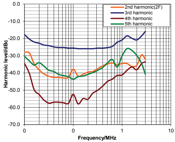
Harmonics
