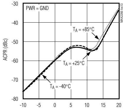
MAX2266 ADJACENT-CHANNEL POWER RATIO vs. OUTPUT POWER
