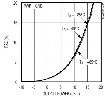
MAX2266 POWER-ADDED EFFICIENCY vs. OUTPUT POWER
