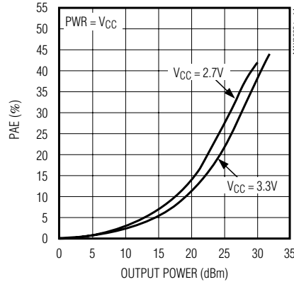
MAX2266 POWER-ADDED EFFICIENCY vs. OUTPUT POWER
