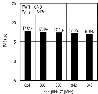
MAX2266 POWER-ADDED EFFICIENCY vs. FREQUENCY
