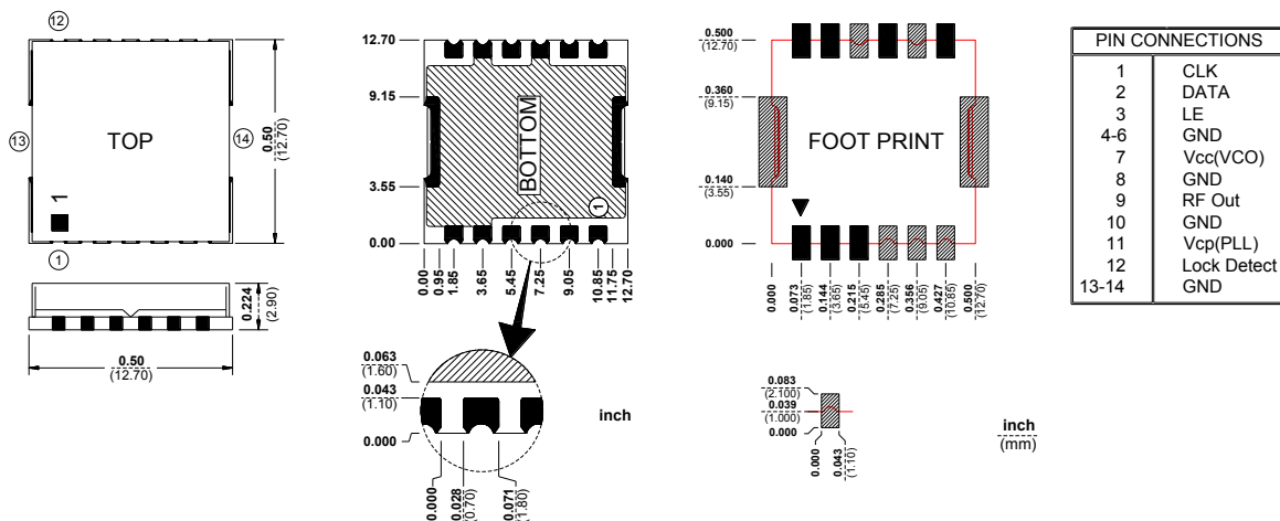
PACKAGE DRAWING : PG12-L
