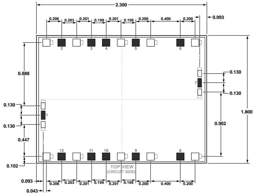
Figure 40. 12-Pad Bare Die [CHIP] (C-12-2) Dimensions shown in millimeter
