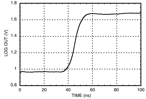
Rise Time @ 10 GHz @ 0 dBm
