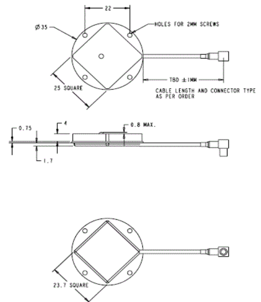
TW1015 Dimensions (mm)
