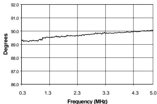
Phase Unbalance
