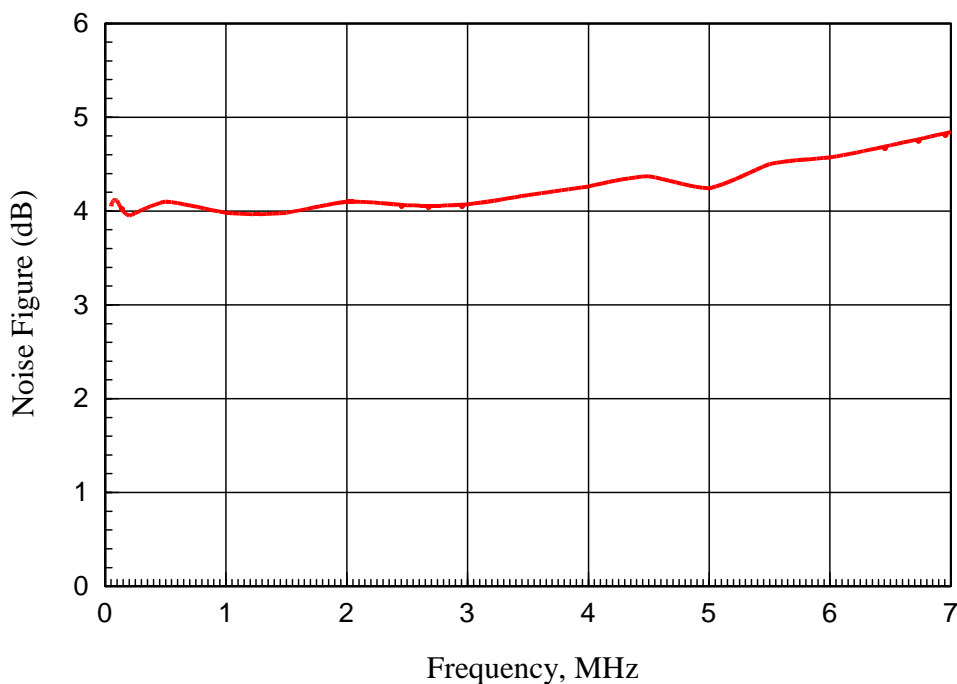
ABL0600-01-2740 Measured Noise Figure vs Frequency
