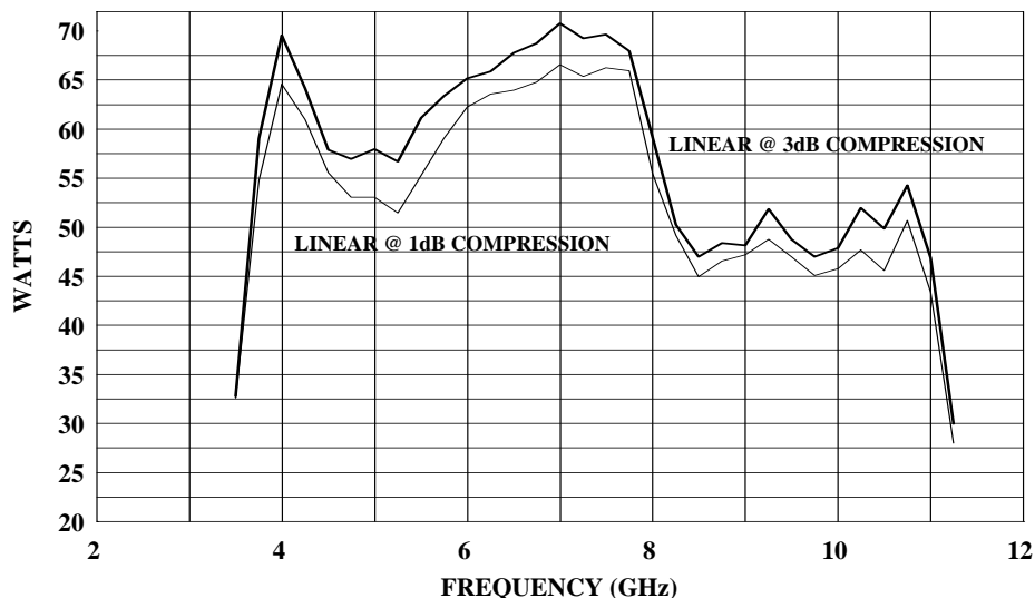
40S4G11 TYPICAL POWER OUTPUT
