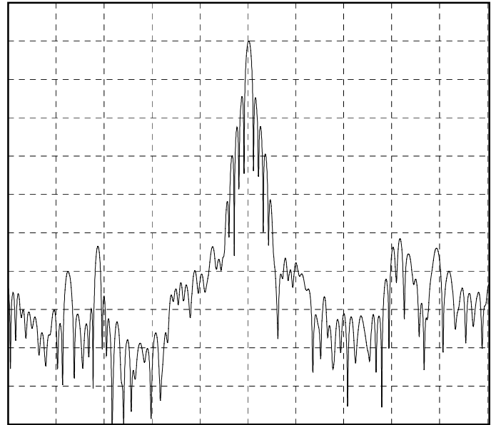
10 dB/div, 0.4 us/div
