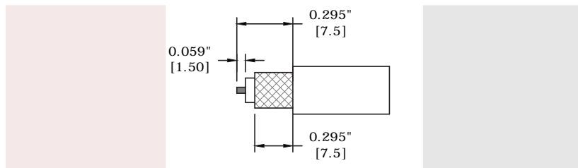
STRIPPING DIMENSION
