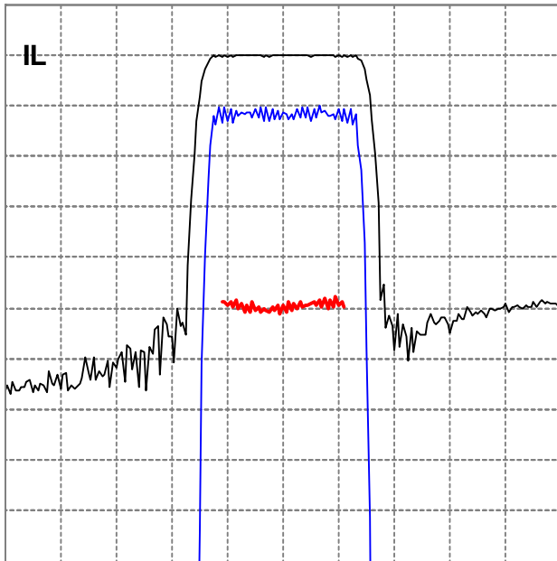
10 dB/div, 1 dB/div, 10 deg/div, 5.000 MHz/div
