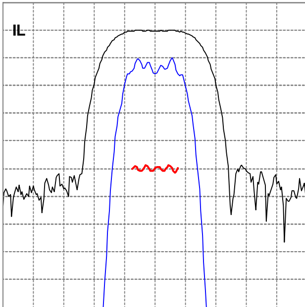
10 dB/div, 1 dB/div, 10 deg/div, 0.300 MHz/div
