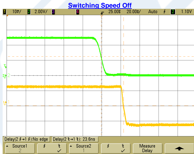
Green Trace: Waveform Generator TTL Levels Yellow Trace: RF Output through mixer IF Port
