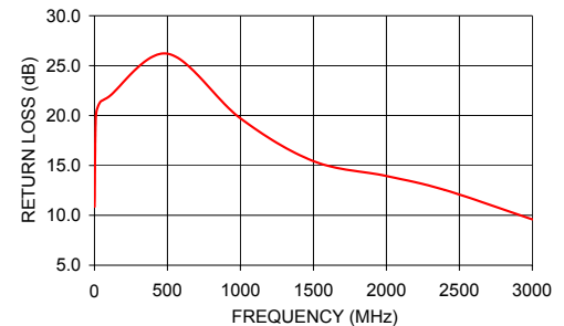
TC1-33-75G2A+ INPUT RETURN LOSS
