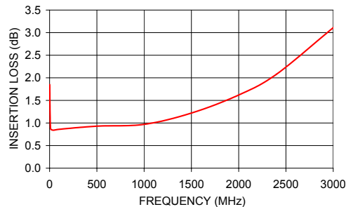
TC1-33-75G2A+ INSERTION LOSS
