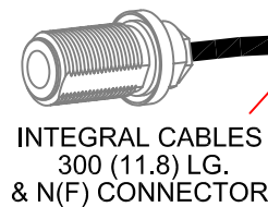
ISOMETRIC VIEW
