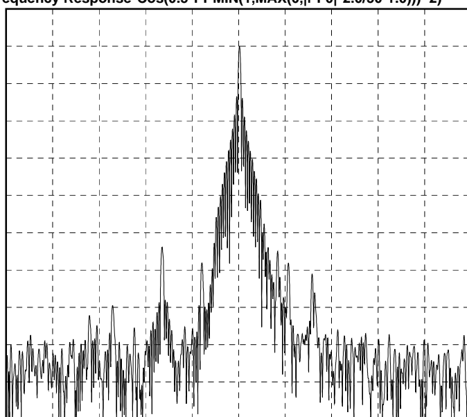
10 dB/div, 0.4 us/div
