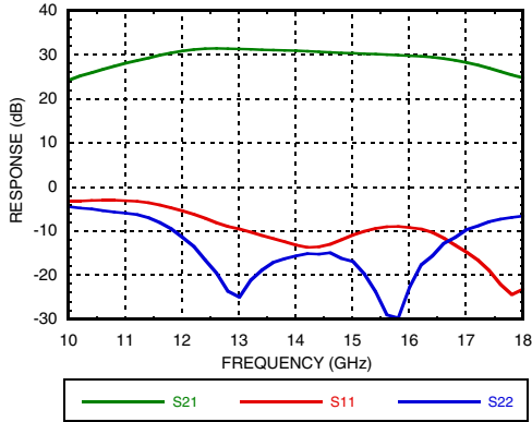
Broadband Gain & Return Loss vs. Frequency
