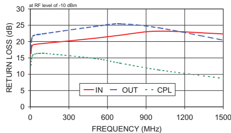
RETURN LOSS
