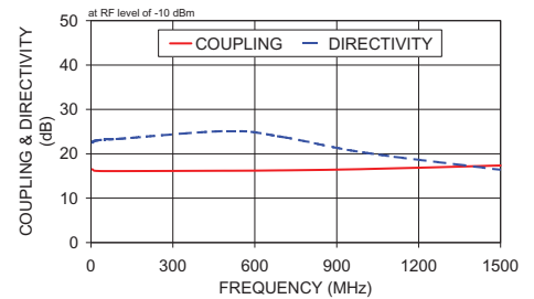
COUPLING & DIRECTIVITY
