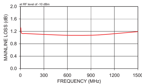
MAINLINE LOSS
