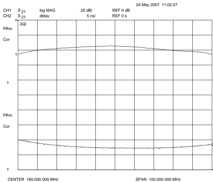
Passband Amplitude & Group Delay (0.25 dB/div and 5 nsec/div)
