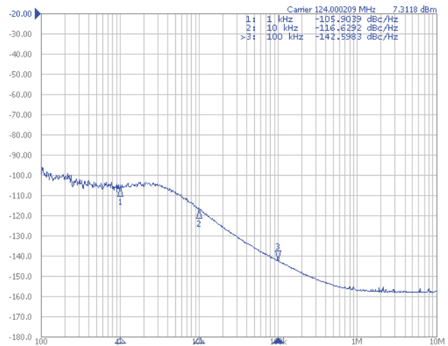
Figure 1: Phase Noise at 124 MHz locked to 10 MHz external reference.
