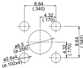
MOUNTING HOLE
