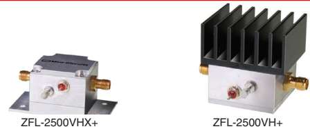
ZFL-2500VHX+ ZFL-2500VH+ CASE STYLE: SS98
