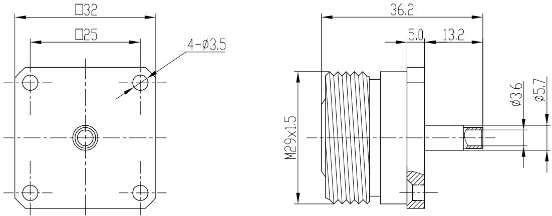
剥线尺寸 stripping dimension
