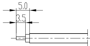
剥线尺寸 stripping dimension
