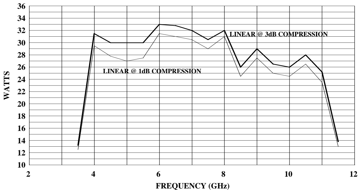
20S4G11A TYPICAL POWER OUTPUT
